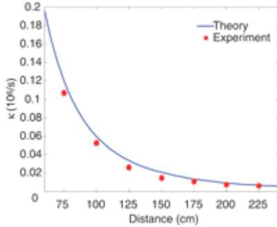
Fig. 2. Comparison of experimental and theoretical values for \kappa as a function of the separation between coaxially aligned source and device coils (the wireless power transfer distance). [View Larger Version of this Image (17K GIF file)]
